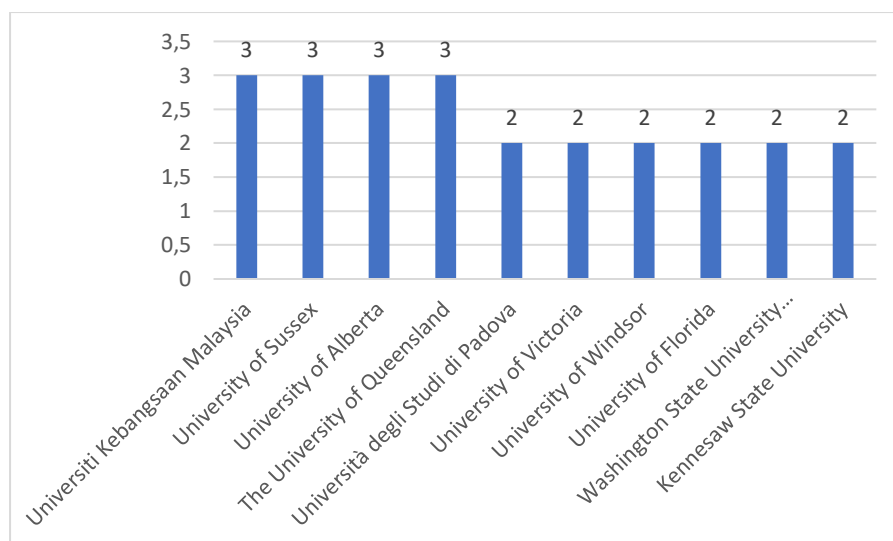
Figure 4. Affiliation Charts
