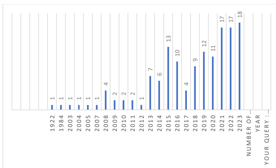
Figure 2. Year Charts
