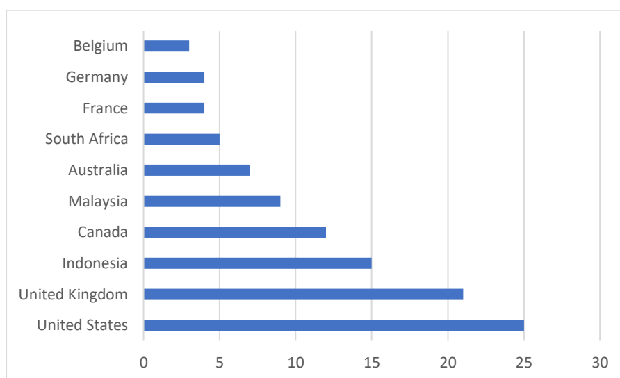
Figure 5. Countries Charts
