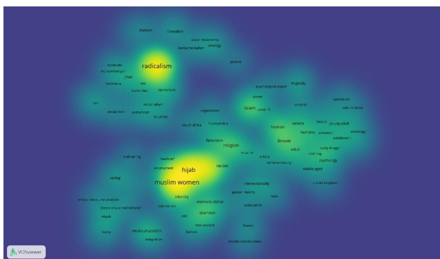
Figure 11. Density Visualisation
