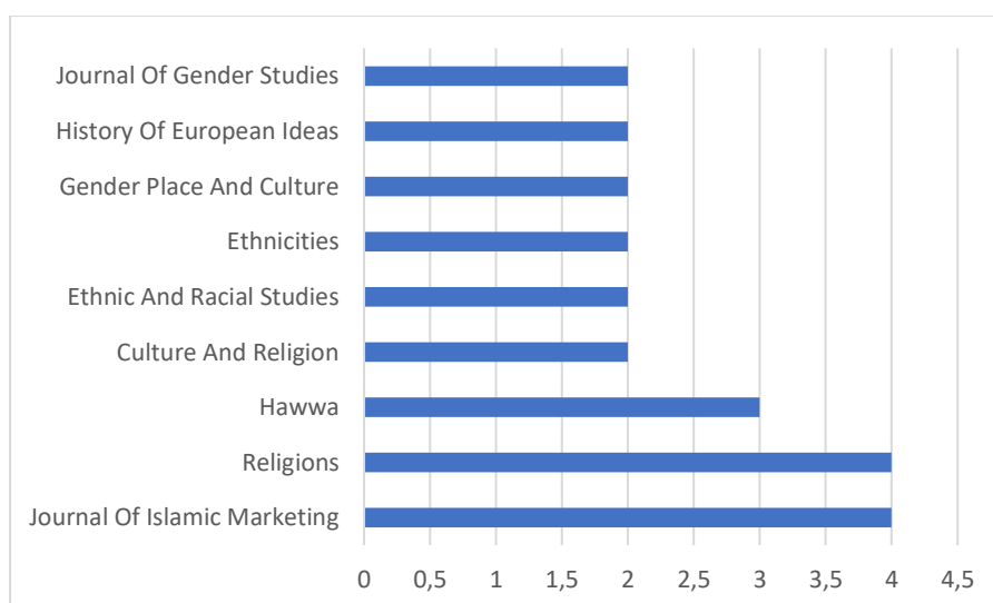
Figure 6. Source Charts
