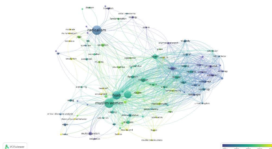
Figure 10. Overlay Visualisation
