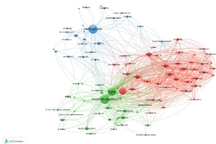
Figure 9. Network Visualisation
