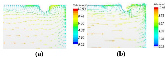
Figure 2: Velocity Vector at The Axisymmetric Plane (a) Continuous Rid (b) Broken-Rib
