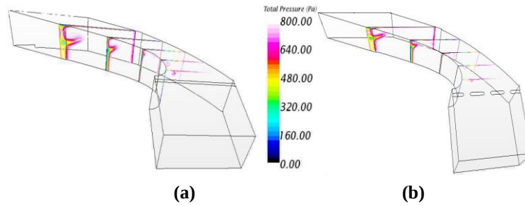
Figure 4: Total Pressure Planes (a) Continuous Rid (b) Broken-Rib
