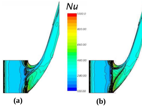
Figure 6: Nusselt Number Distribution at The Endwall (a) Broken-Rib (b) Continuous-Rid
