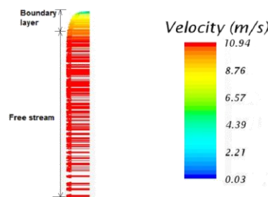
Figure 1: Inlet Velocity Profile
