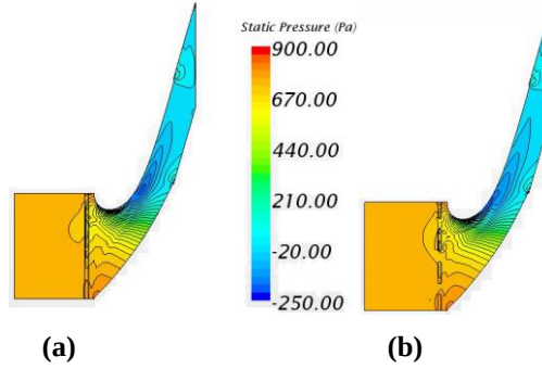
Figure 3: Static Pressure Distribution at The Endwall (a) Continuous Rid (b) Broken-Rib
