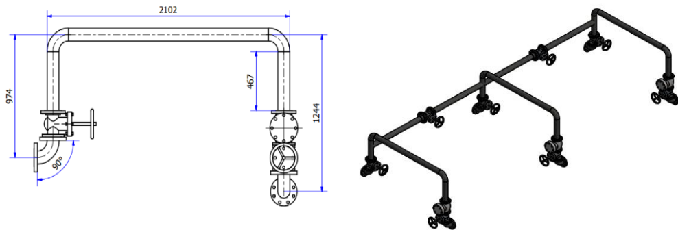
Figure 1. Basic Pipeline Compressors in Power Plant Tanjung Enim 3x10 MW
