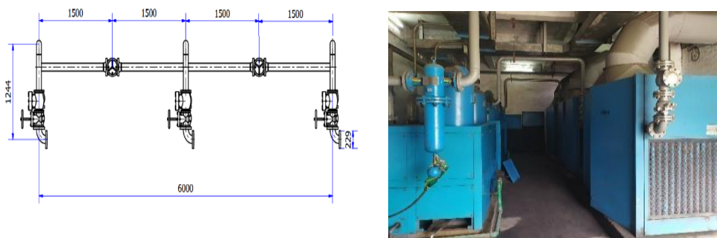
Figure 2. Plan of Modification Pipeline Compressors in Power Plant Tanjung Enim 3x10 MW
