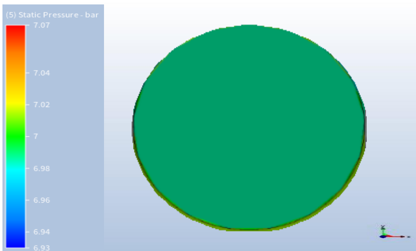
Figure 10. Pressure Outlet Section Distribution Modification Pipeline
