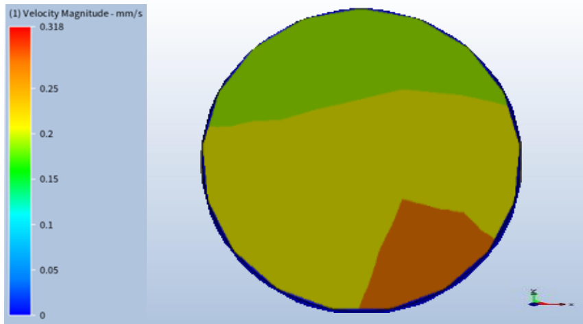
Figure 13. Velocity outlet section distribution of Basic Pipeline
