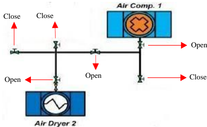
Figure 4. Modification Schematic Analysis compressor pipeline system
