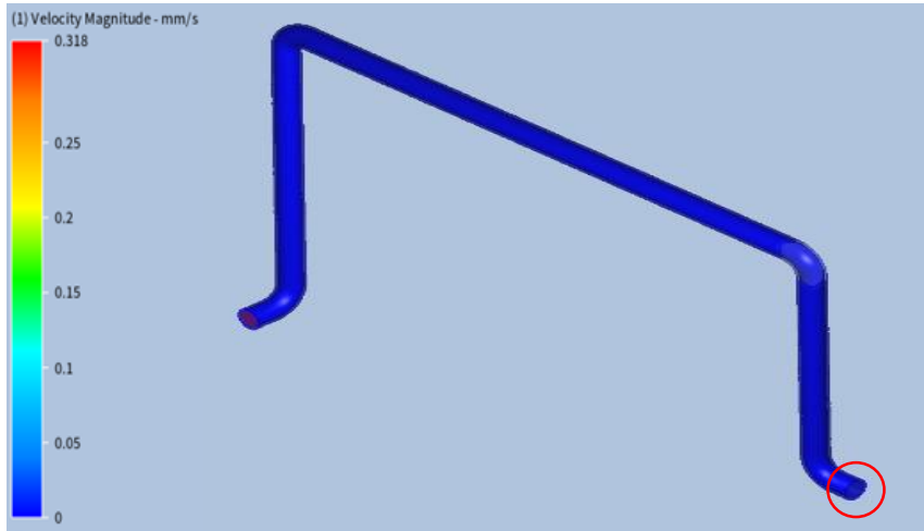
Figure 11. Velocity analysis of Basic Pipeline
