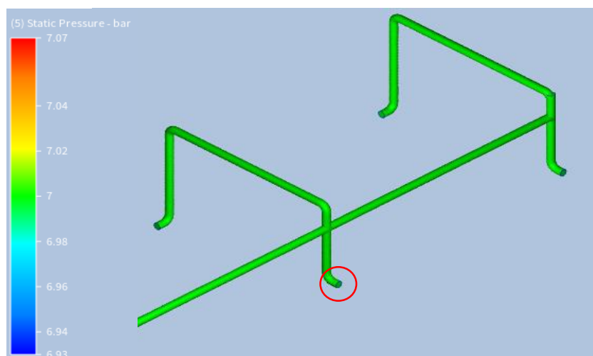
Figure 8. Modification Pipeline Pressure Analysis
