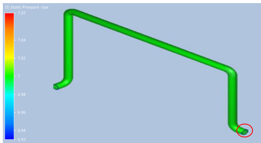
Figure 7. Basic Pipeline Pressure Analysis
