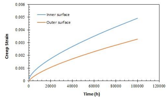
Figure 4. Development of creep strain.
