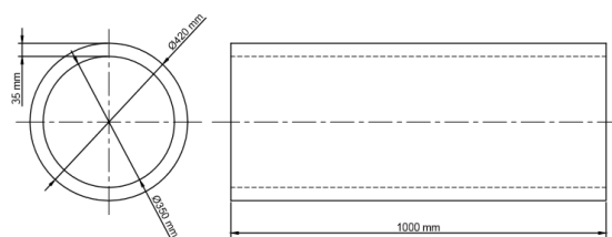
Figure 1. Schematic model of pipe.
