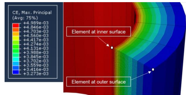
Figure 3. Location of elements at the inner and outer pipe surface.
