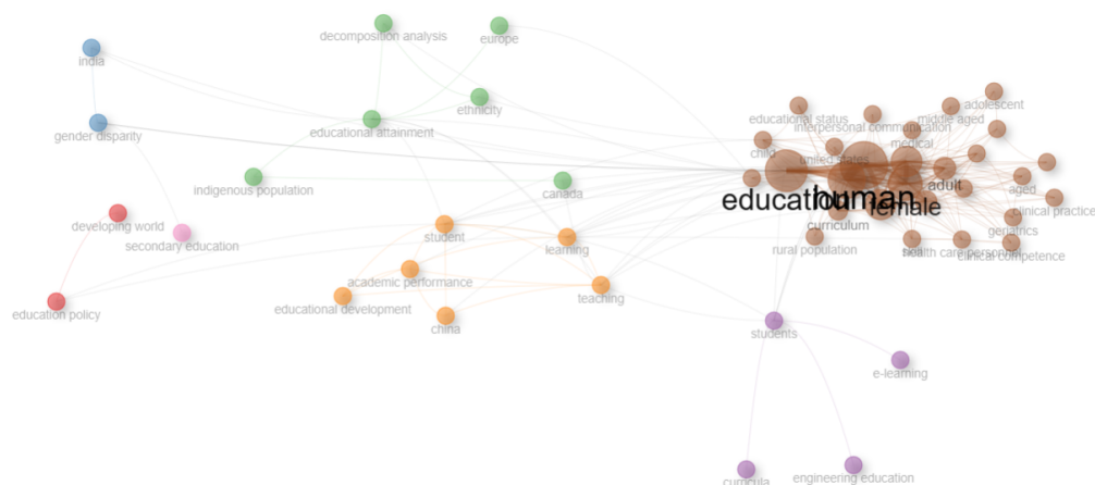
Figure 5. Co-occurrence Network
