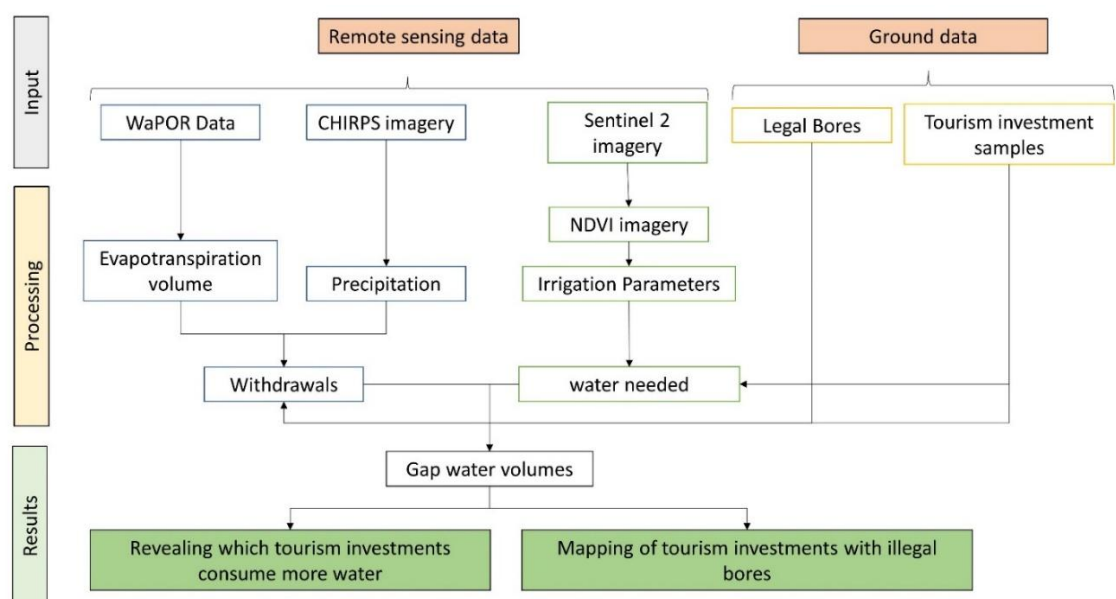
Figure 2. Methodology diagram.
