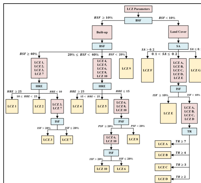
Figure 3. The Hierarchical Decision Tree for GIS-Based Rule Classification of LCZ.
