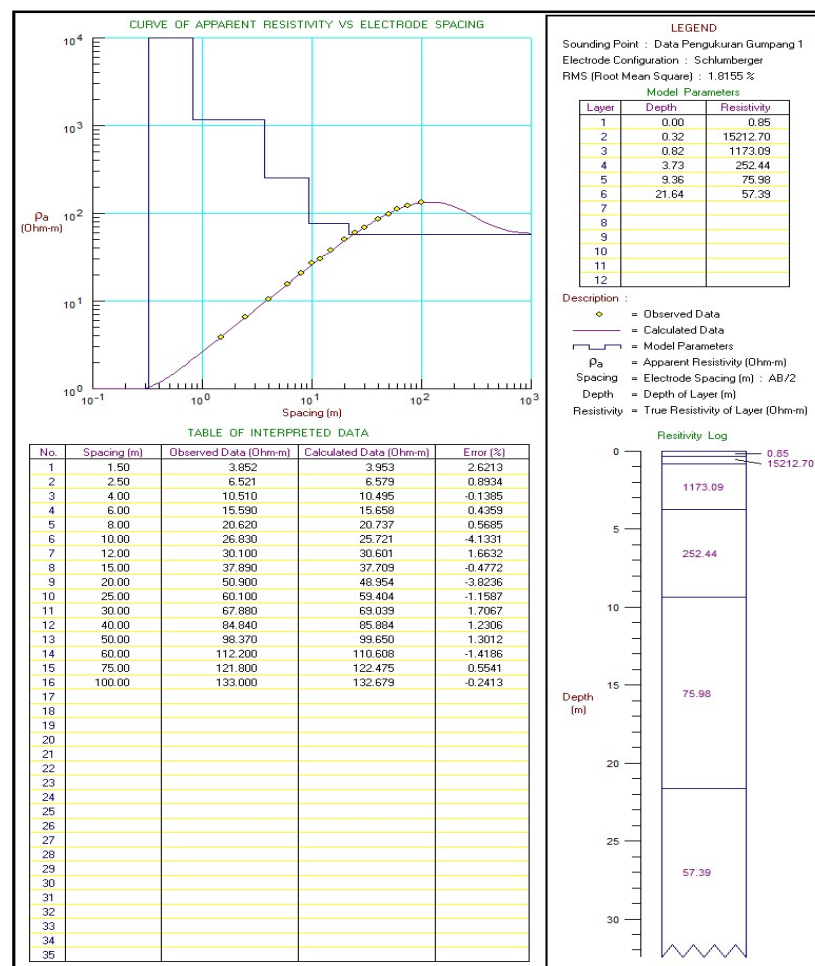
Figure 4. Resistivity Value of Point 1
